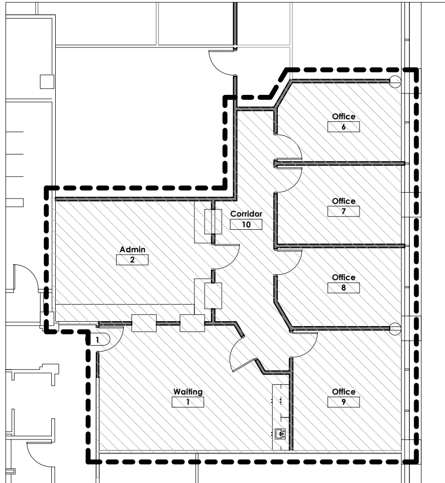
1 Renovation Plan with Sublease A202 1/8" = 1'-0"
